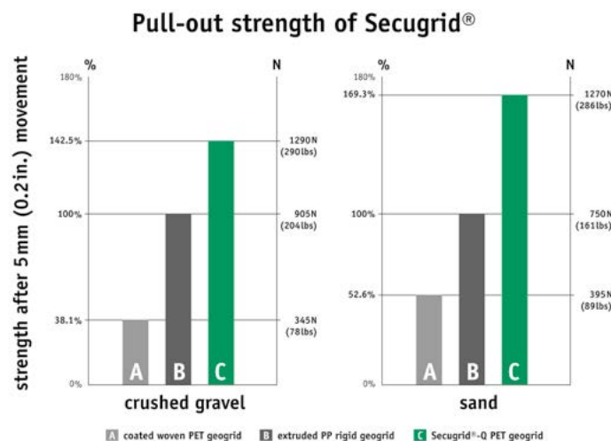
Fig. 15 Soil pull-out results with 3 geogrids
