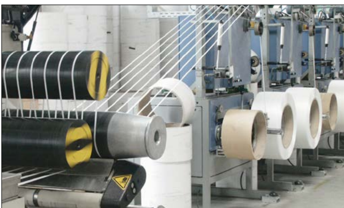
Fig. 4 Stretching process of Secugrid® ribs
