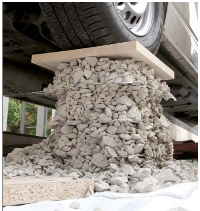
Fig. 10 Demonstration of the interlock effect with a car standing on a Secugrid® reinforced gravel column
